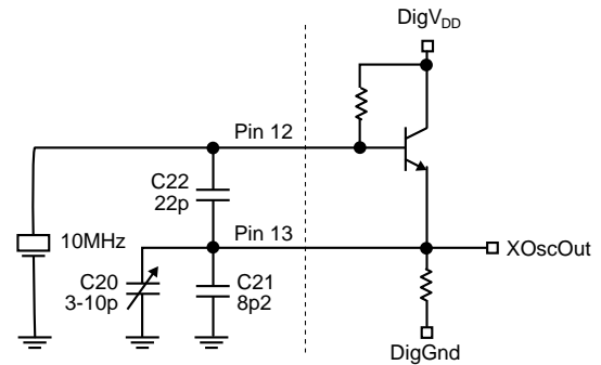
Figure 5. Crystal Oscillator
