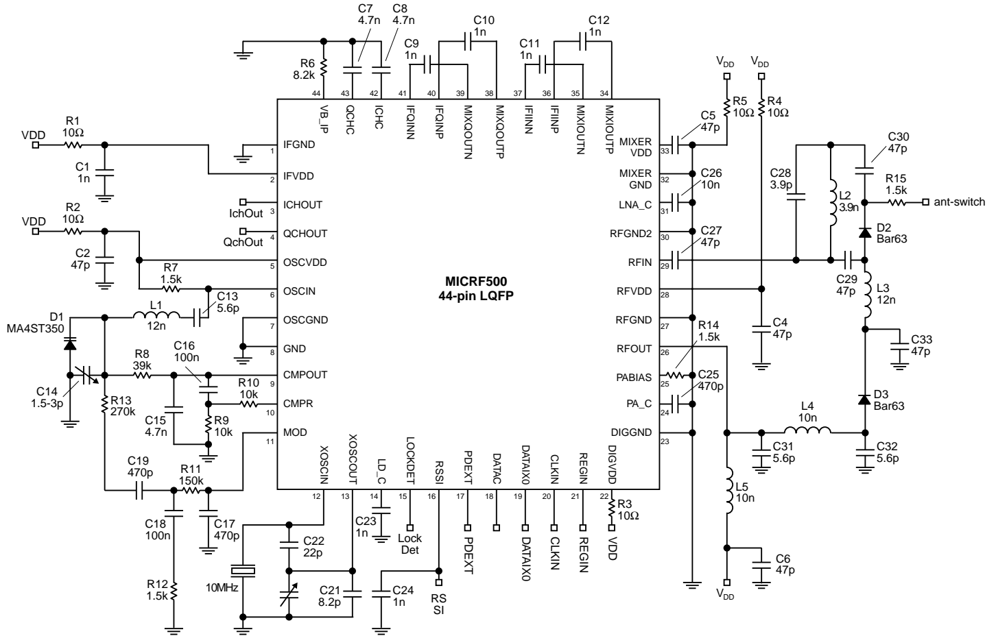
Figure 3. Application Circuit
