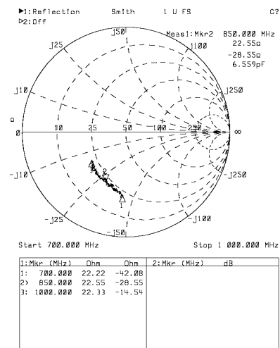
Figure 9. Input Impedance
