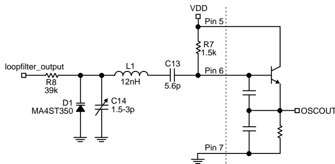
Figure 4. VCO
