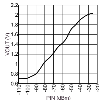
Figure 10. Typical RSSI Characteristics
