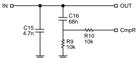
Figure 7. Second Order Loop Filter
