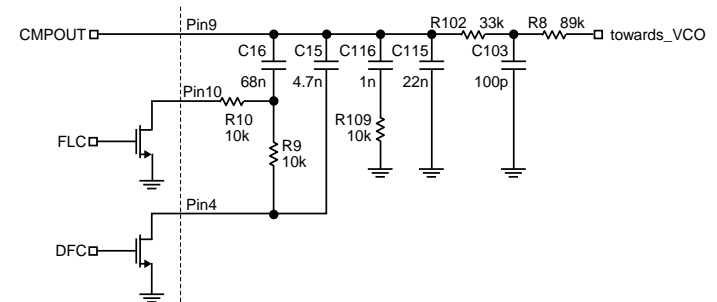
Figure 8. Dual Loop-Filters
